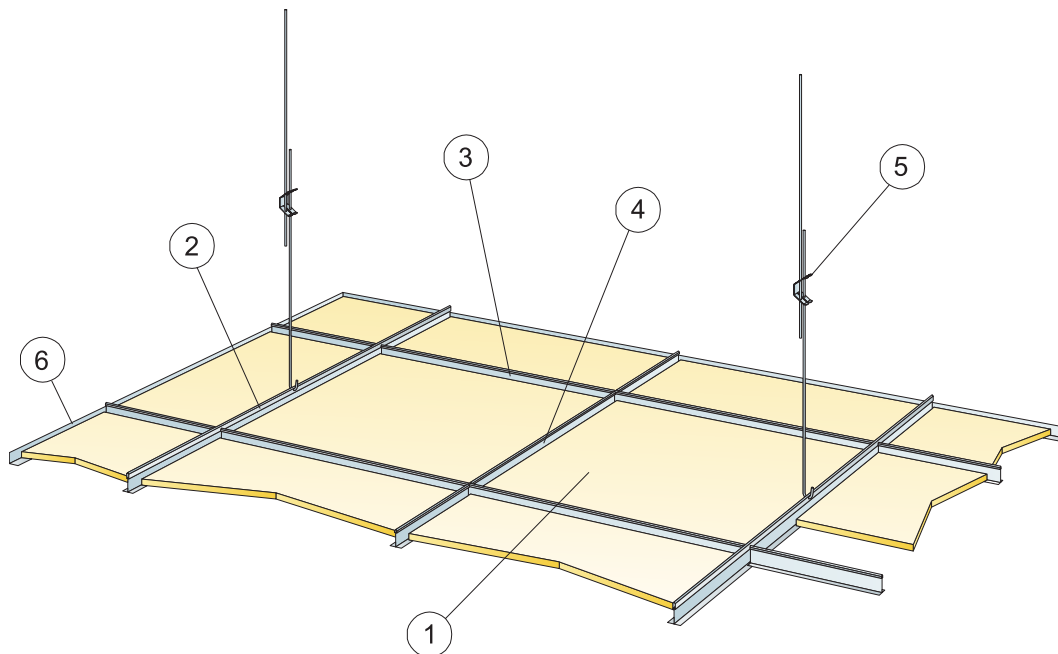
Installation diagram (M360) for Ecophon Opta A
